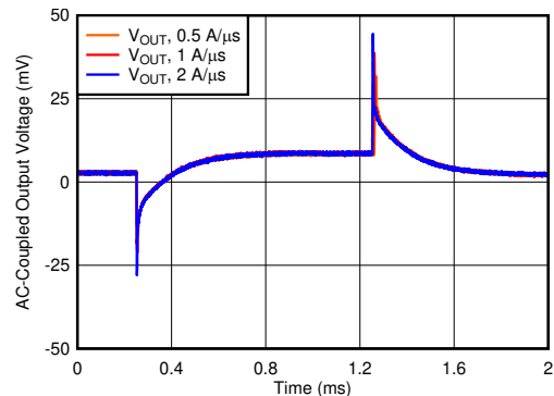
V_{OUT} = 5\text{ V} , I_{OUT,DC} = 100\text{ mA} , I_{OUT} = 100\text{ mA} to 3\text{ A} , C_{OUT} = 47\text{ }\mu\text{F} \parallel 10\text{ }\mu\text{F} \parallel 10\text{ }\mu\text{F} , C_{NR/SS} = C_{FF} = 10\text{ nF}
